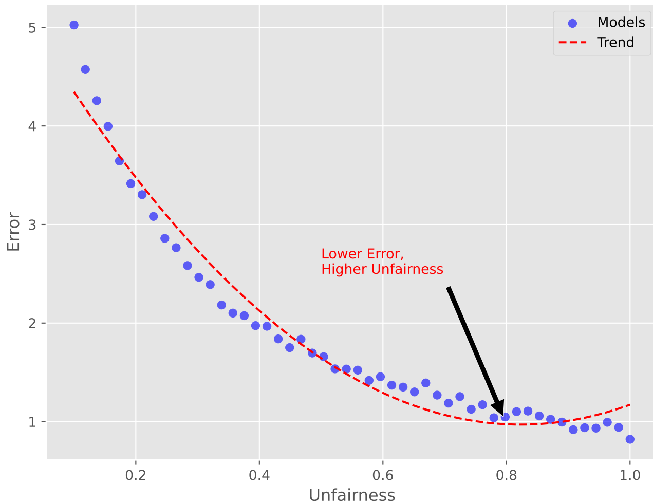
Tradeoff between Error and Unfairness
